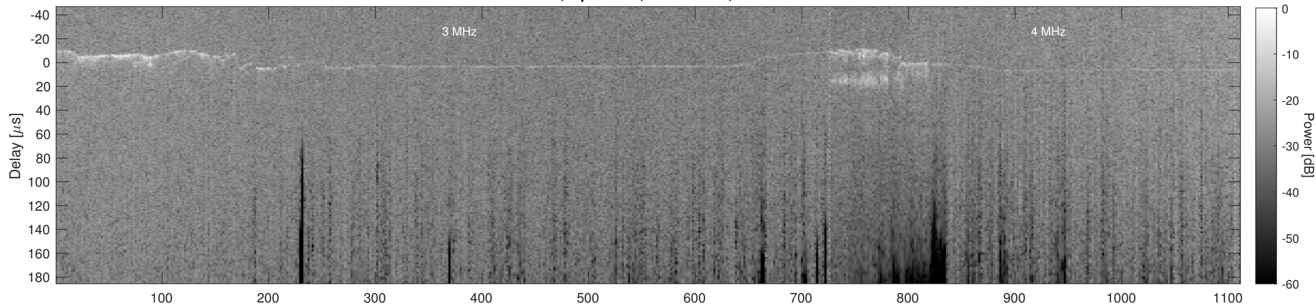
Orbit 9880, Cluttergram
