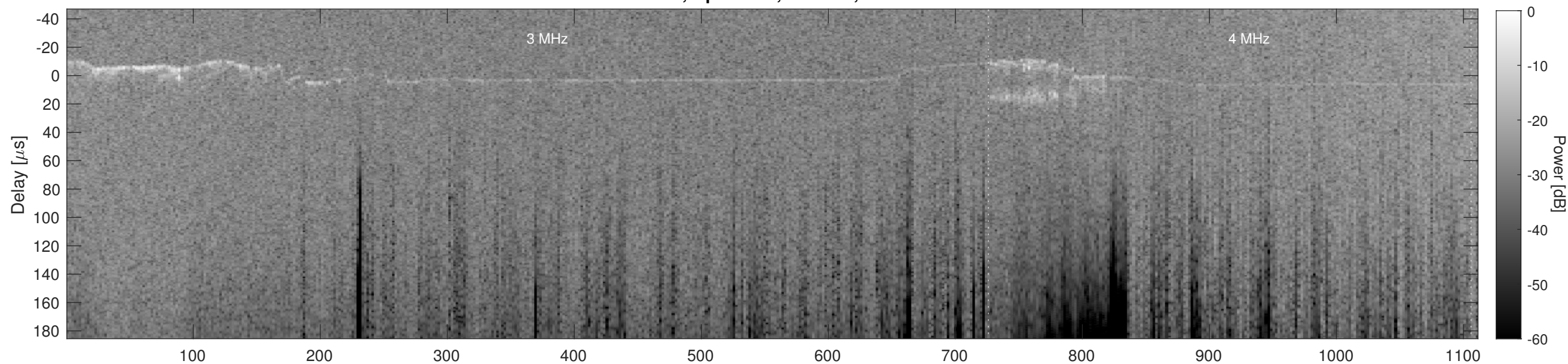
Orbit 9880, Cluttergram
