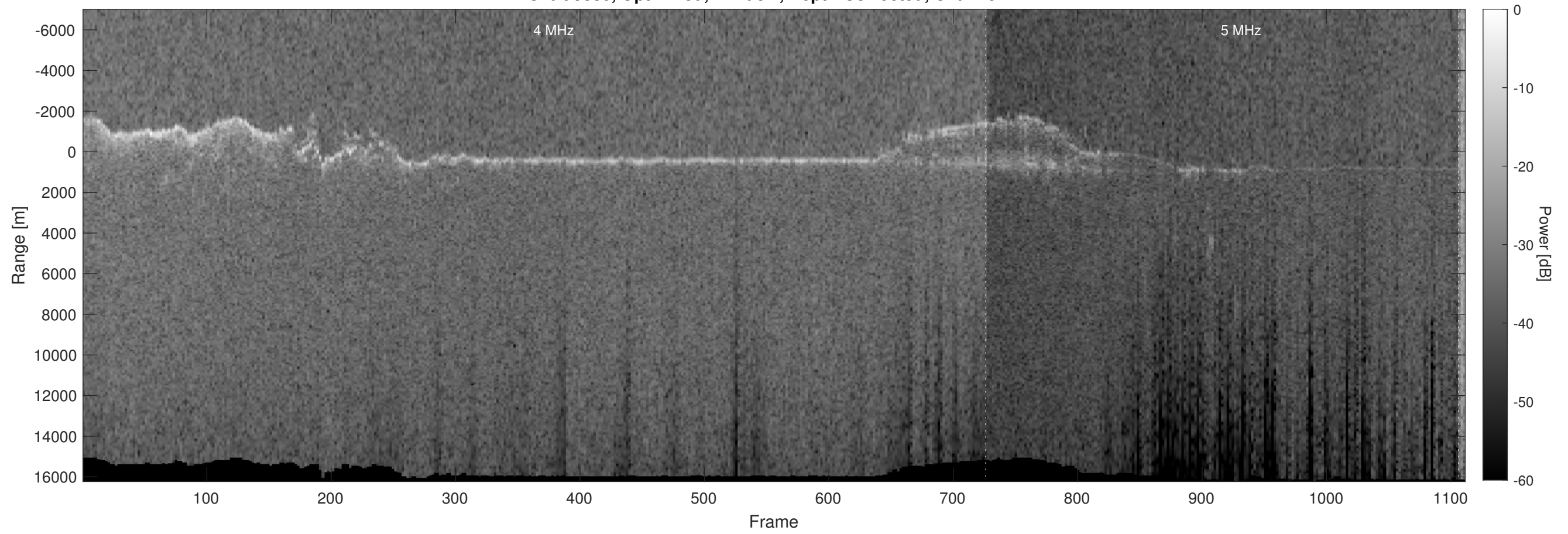
Orbit 9880, Optimized, Window, Depth-Corrected, Channel 2
