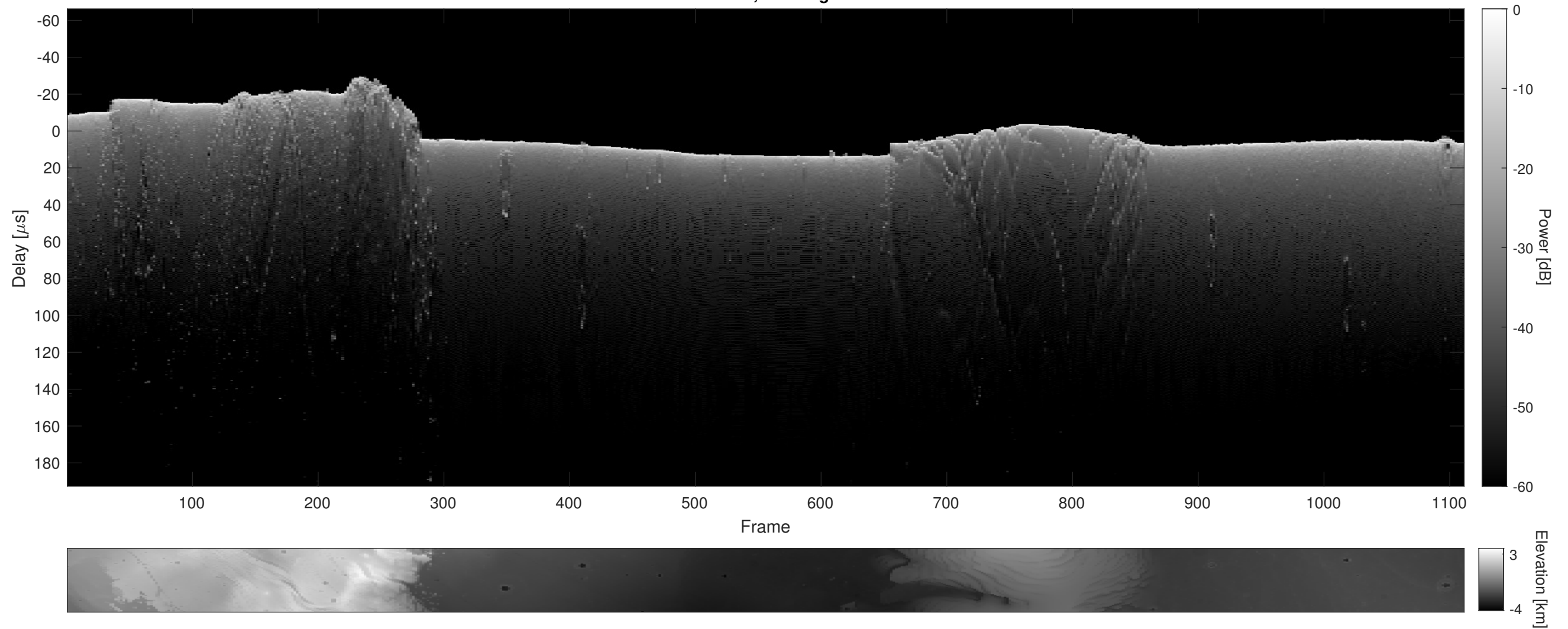
Orbit 9881, Cluttergram
