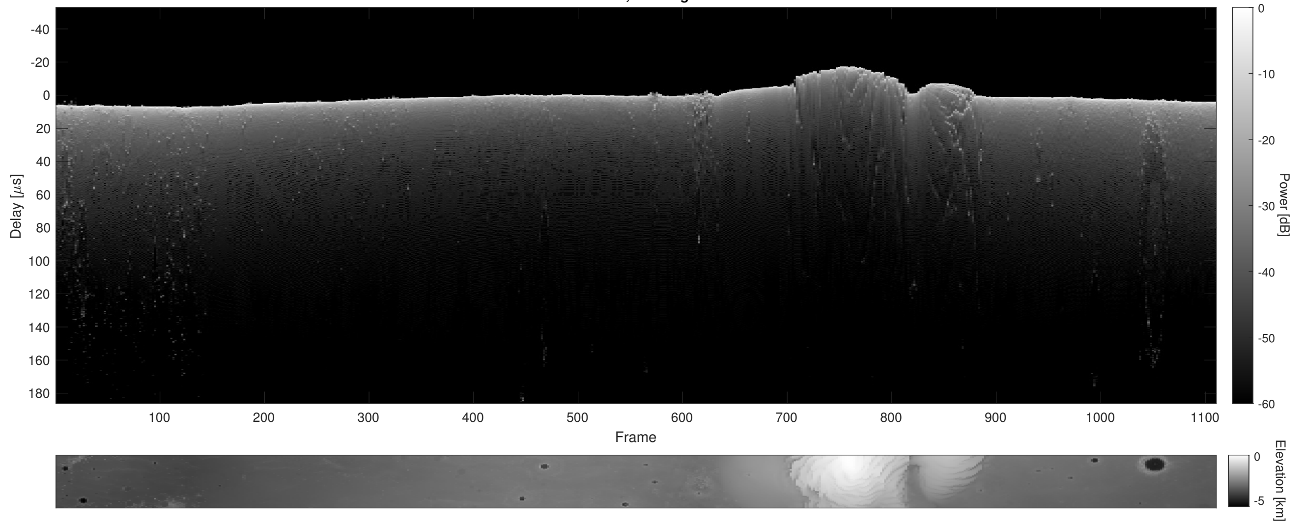
Orbit 9882, Cluttergram
