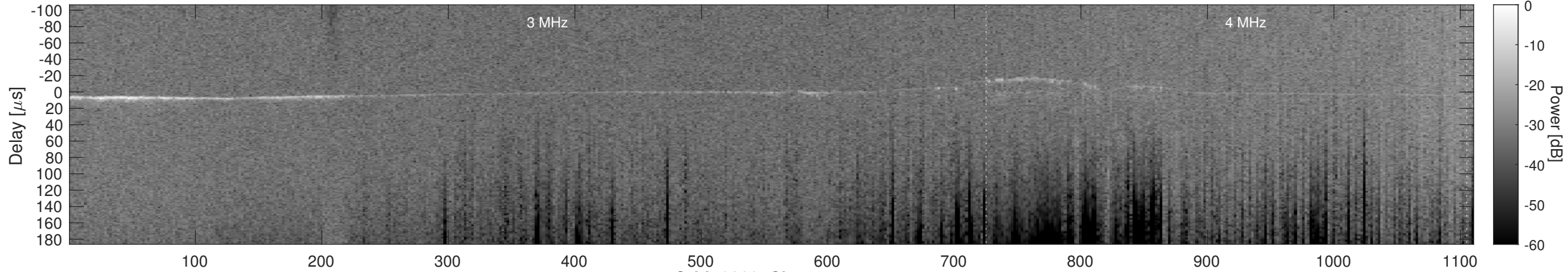
Orbit 9882, Cluttergram
