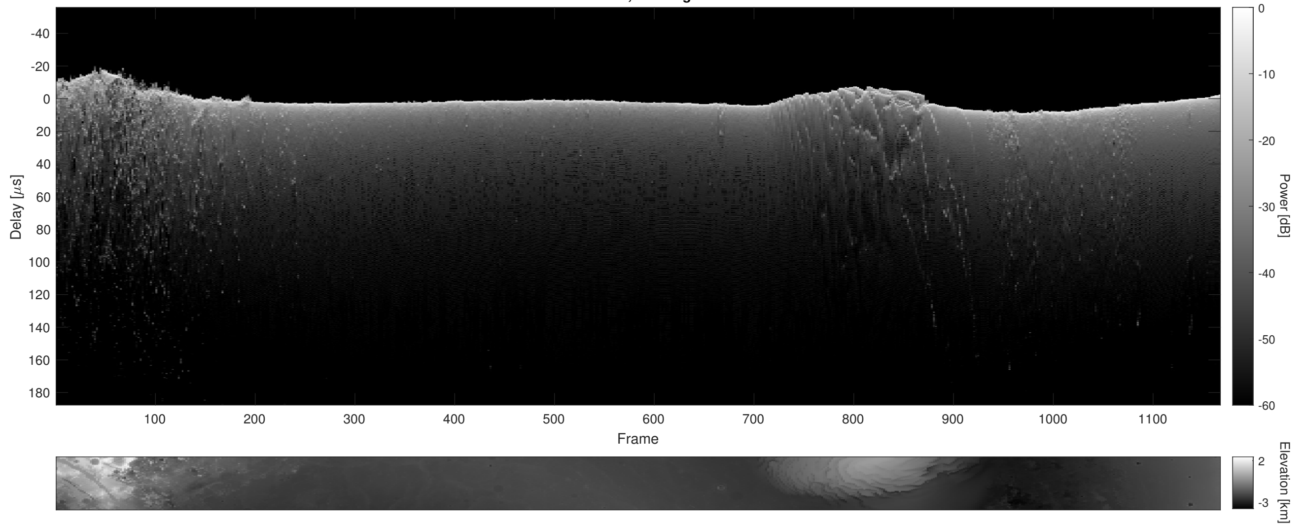
Orbit 9883, Cluttergram
