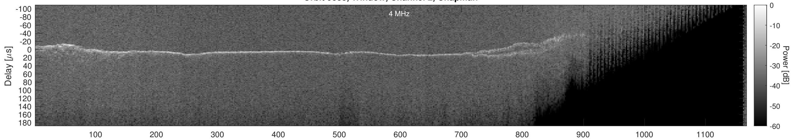
Orbit 9883, Window, Channel 2, Optimized
