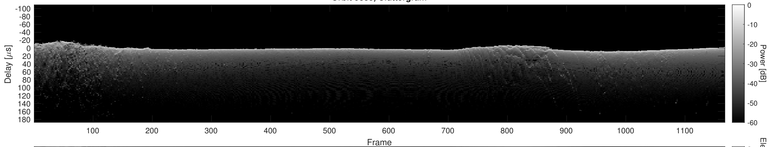
Orbit 9883, Cluttergram
