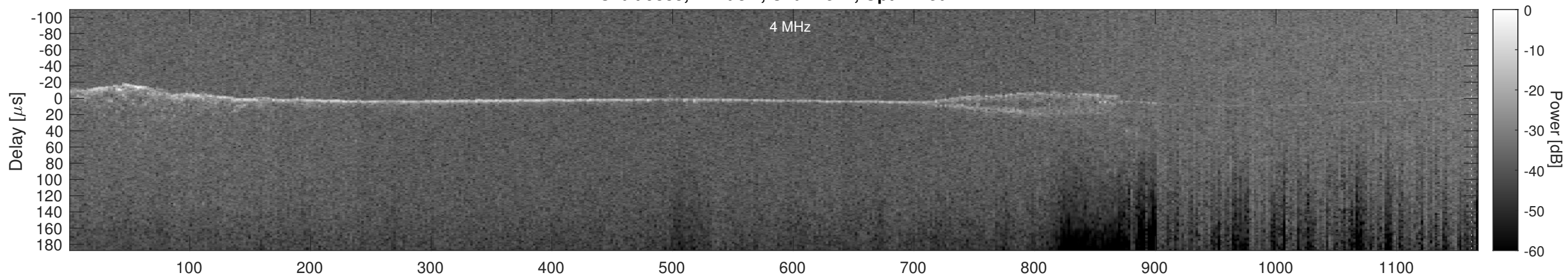
Orbit 9883, Cluttergram
