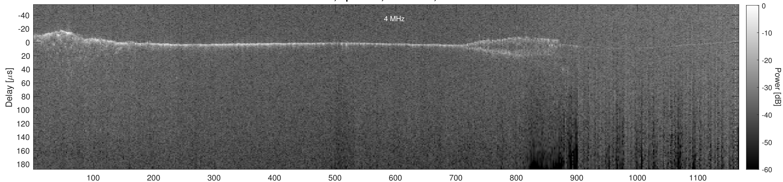
Orbit 9883, Cluttergram
