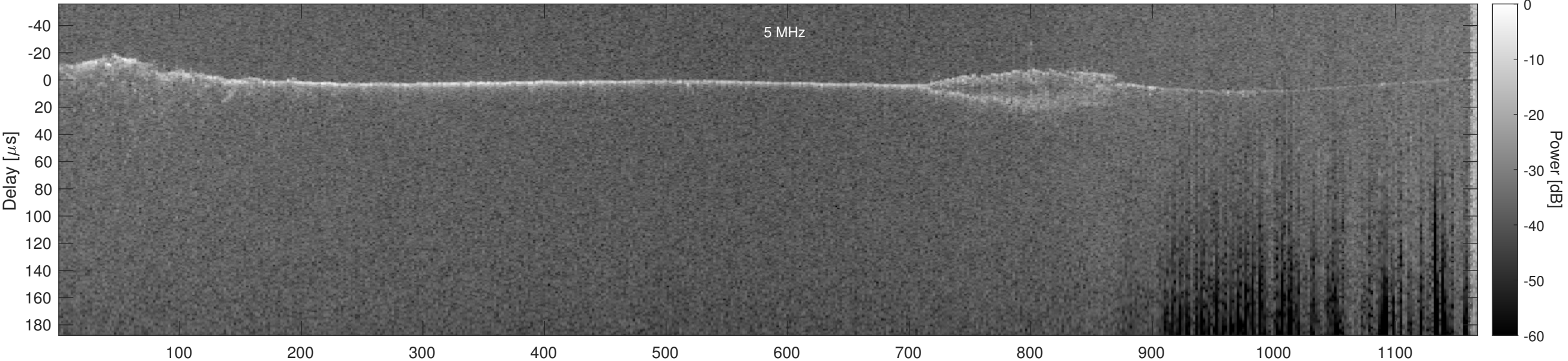
Orbit 9883, Optimized, Window, Channel 2
