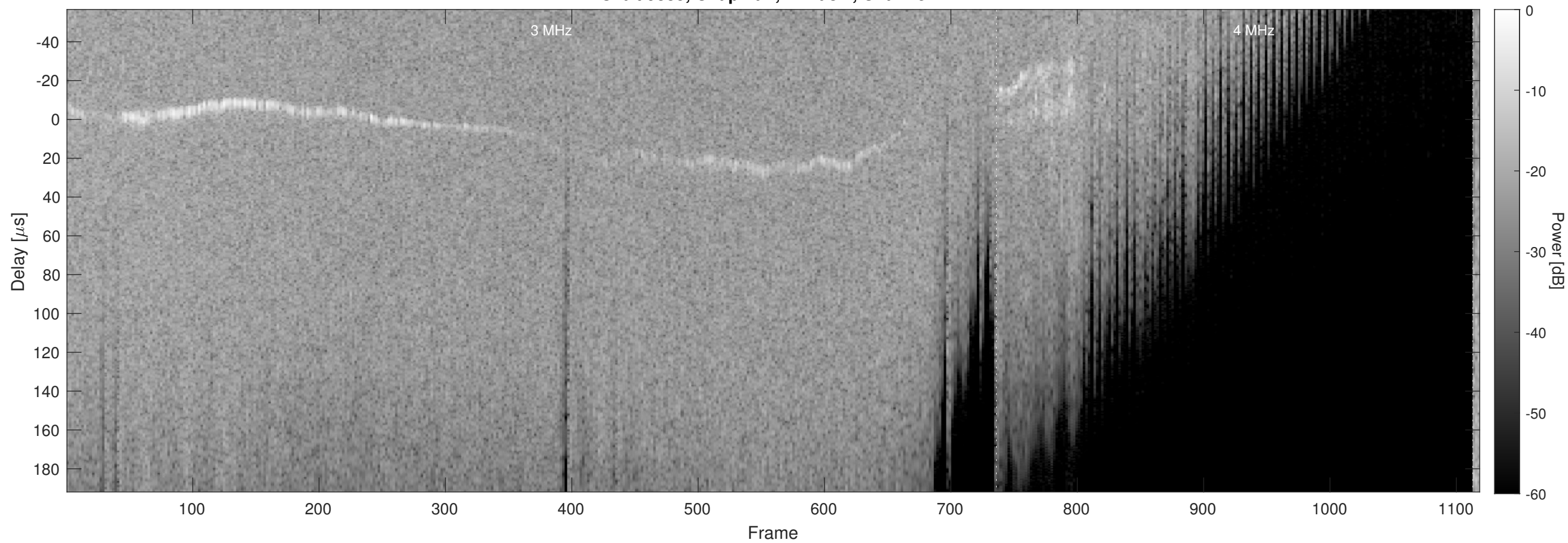
Orbit 9885, Chapman, Window, Channel 2
