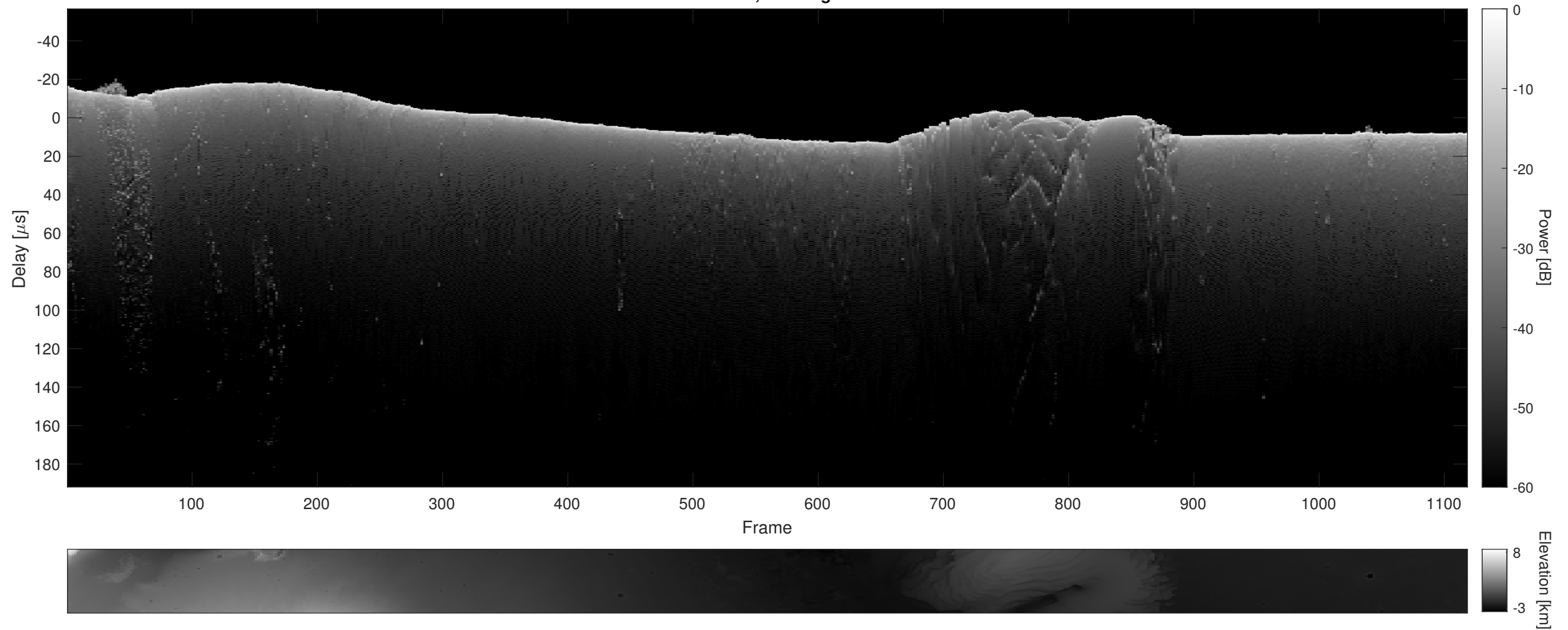
Orbit 9885, Cluttergram
