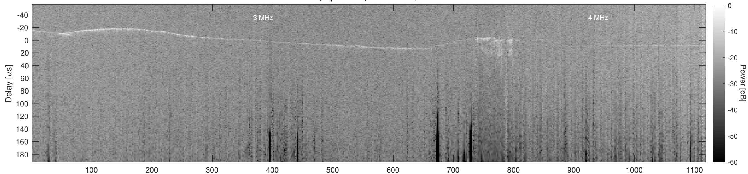
Orbit 9885, Cluttergram
