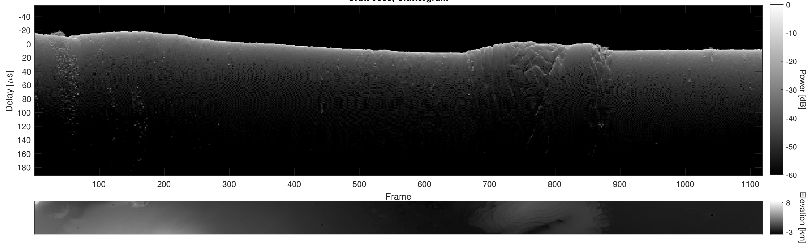
Orbit 9885, Cluttergram
