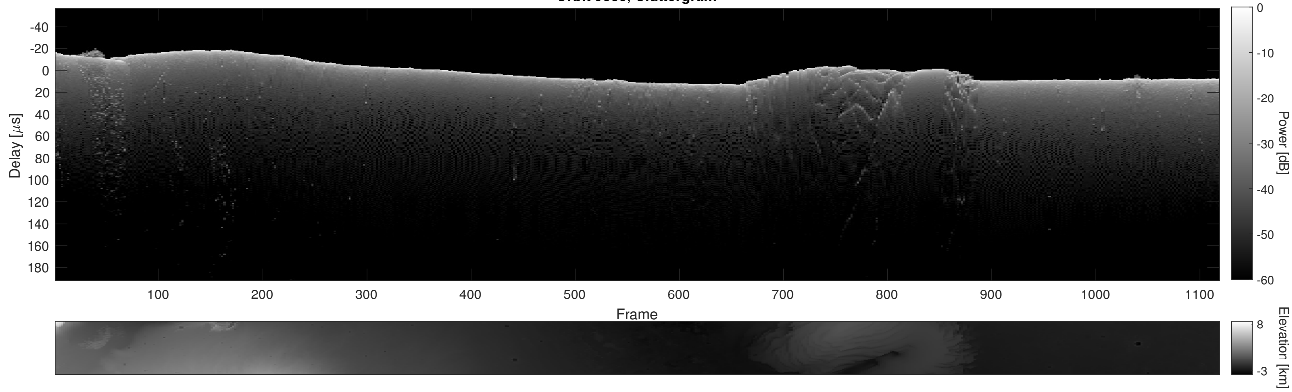
Orbit 9885, Cluttergram
