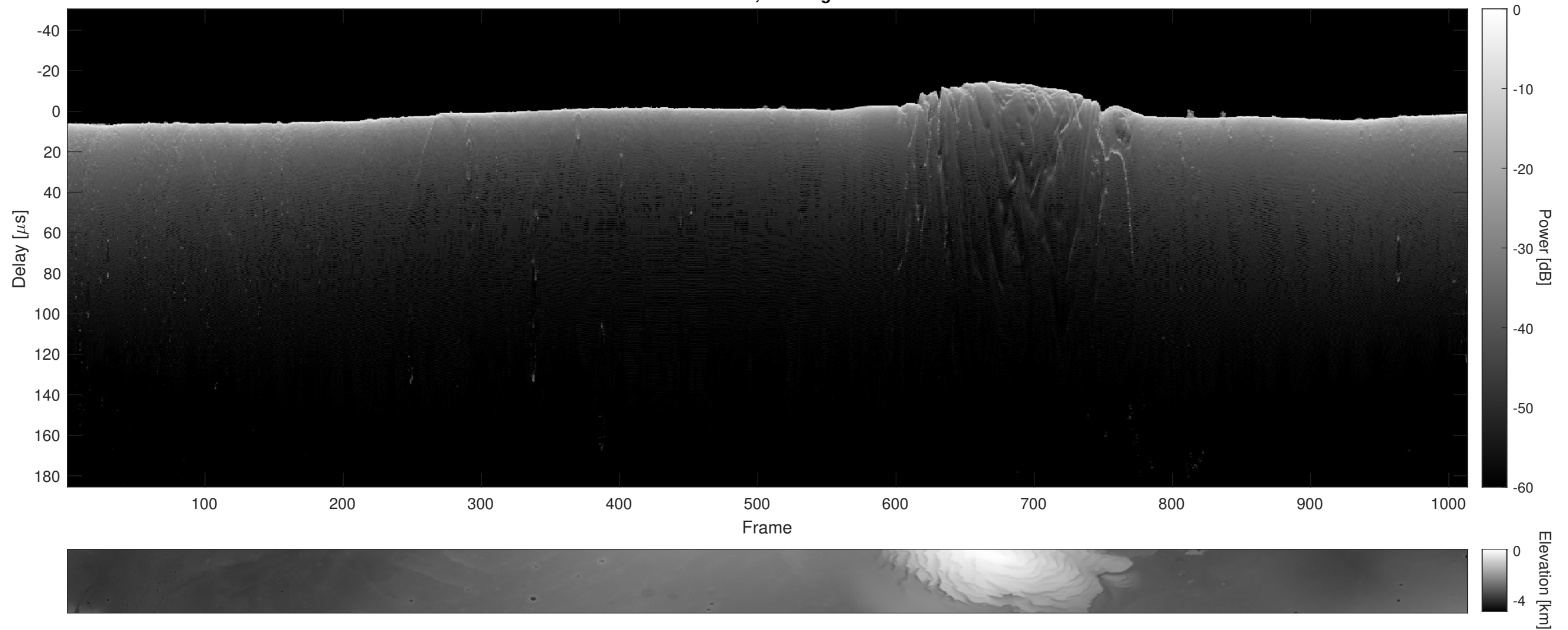
Orbit 9886, Cluttergram
