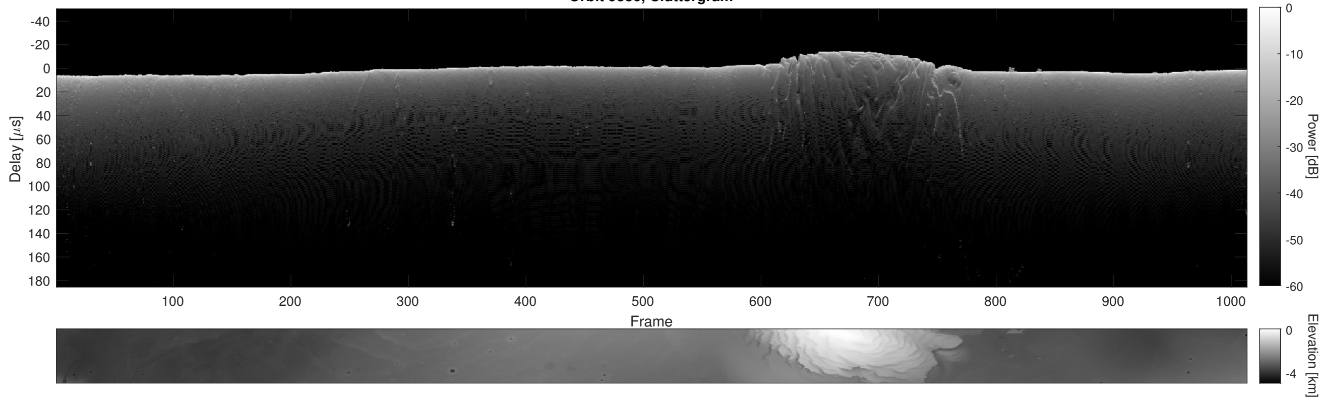
Orbit 9886, Cluttergram
