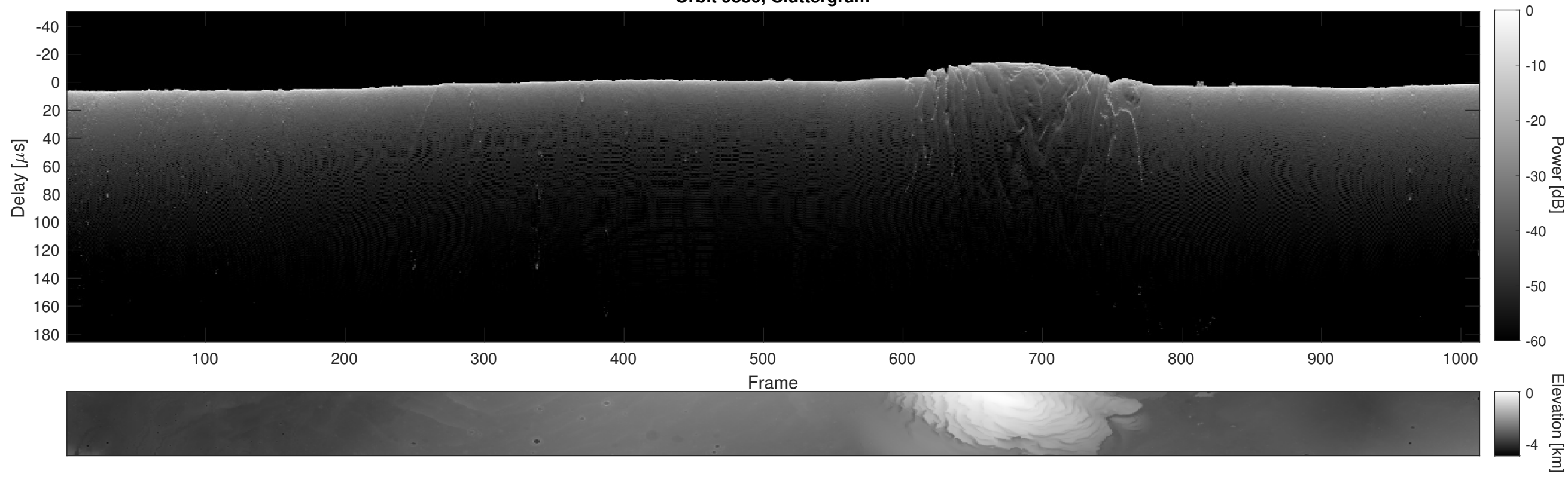
Orbit 9886, Cluttergram
