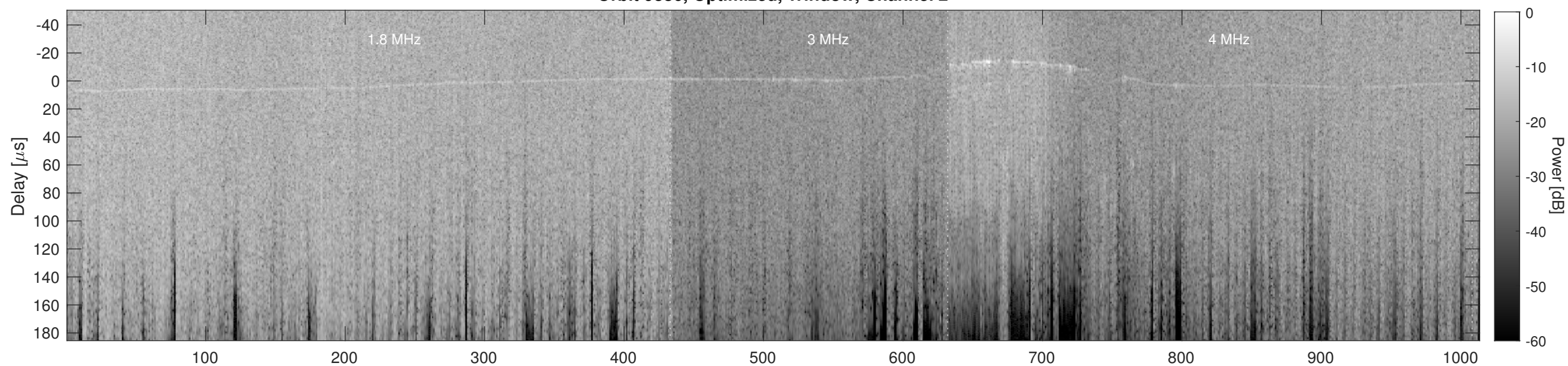
Orbit 9886, Cluttergram
