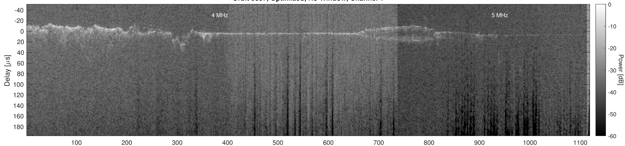
Orbit 9887, Optimized, No Window, Channel 2
