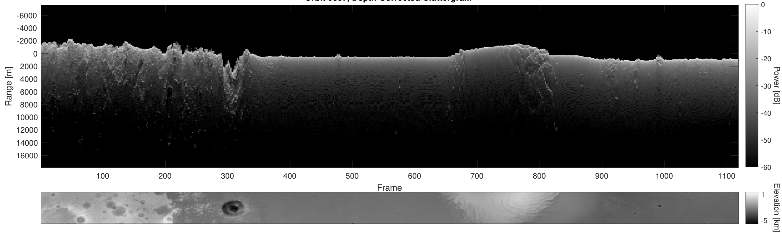
Orbit 9887, Depth-Corrected Cluttergram
