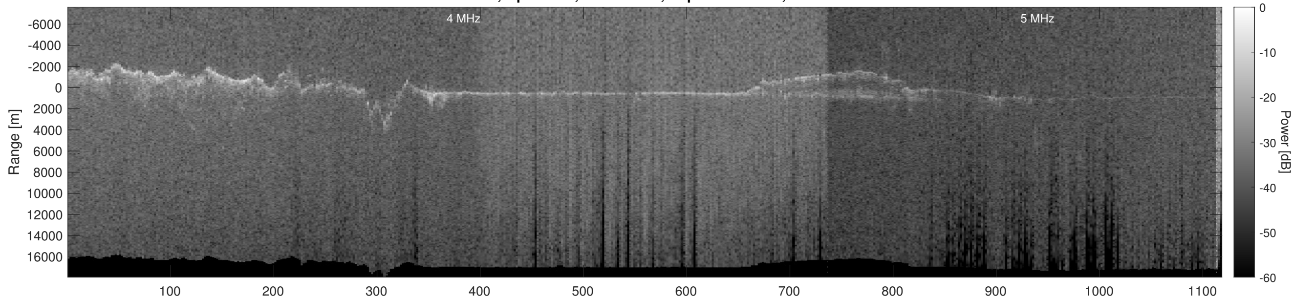
Orbit 9887, Optimized, No Window, Depth-Corrected, Channel 2
