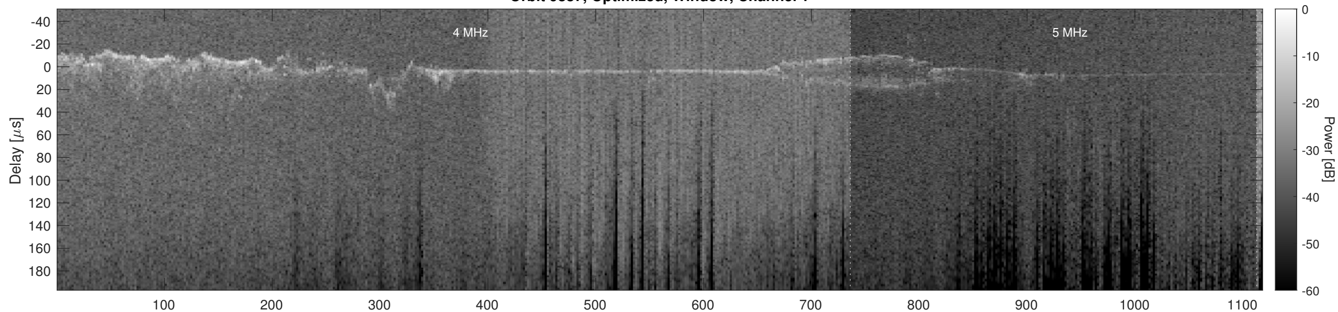
Orbit 9887, Optimized, Window, Channel 2
