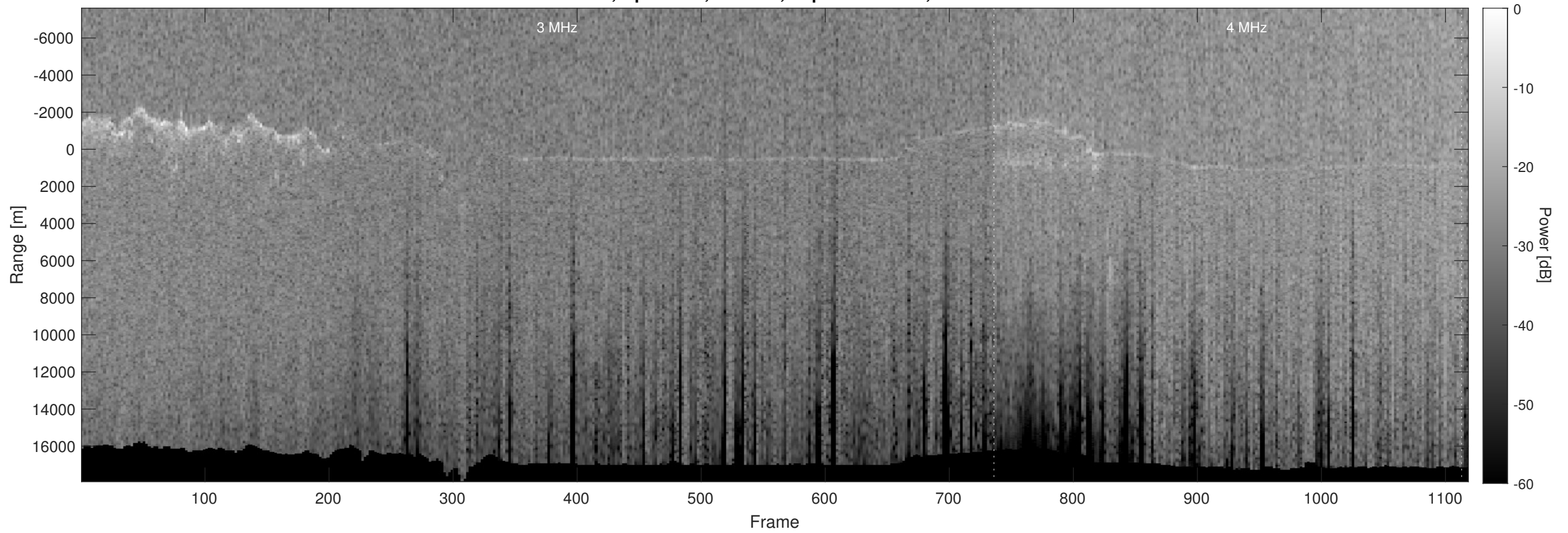
Orbit 9887, Optimized, Window, Depth-Corrected, Channel 2
