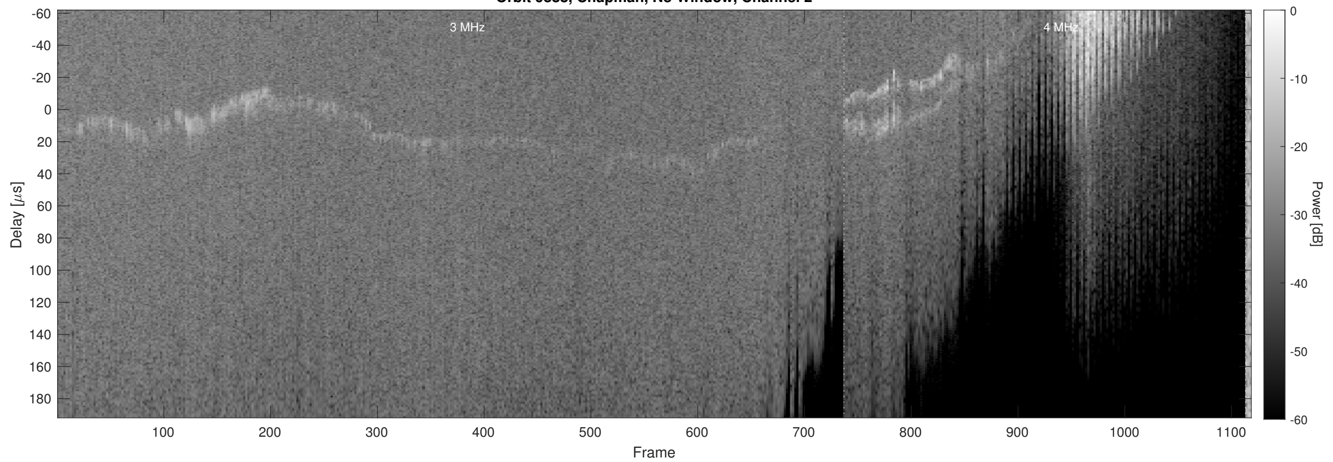
Orbit 9888, Chapman, No Window, Channel 2
