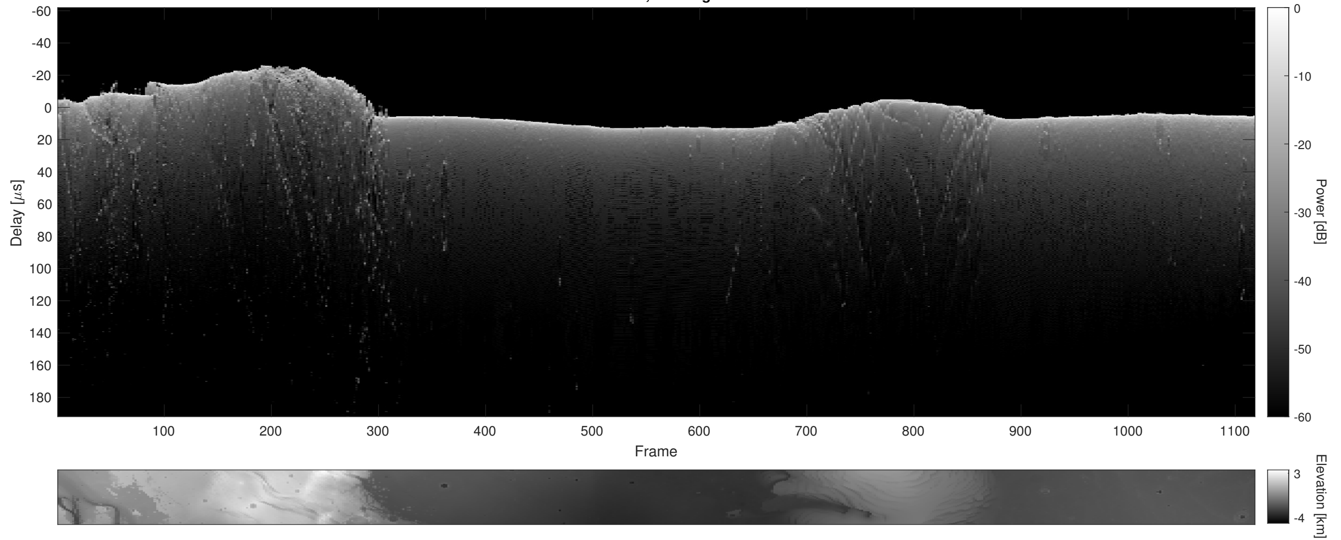
Orbit 9888, Cluttergram
