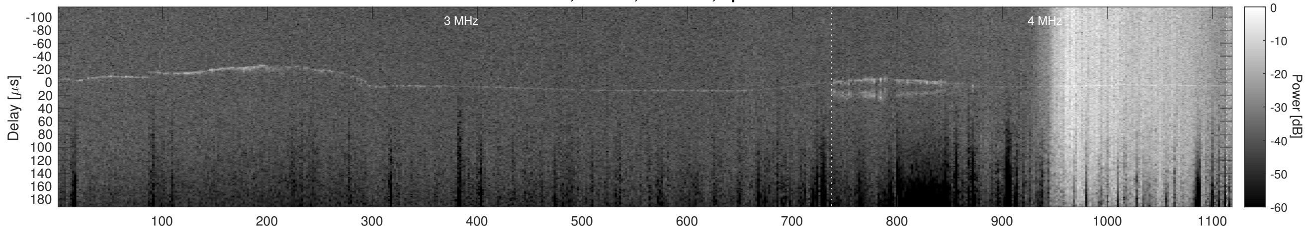
Orbit 9888, Cluttergram
