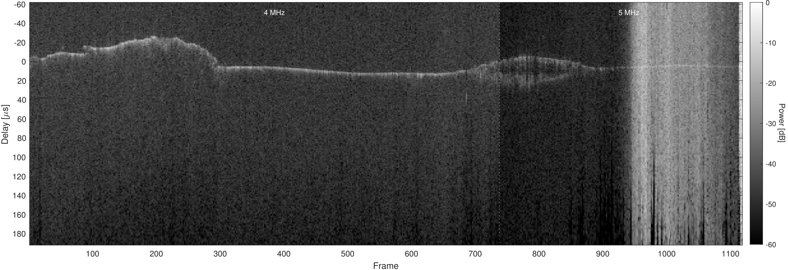
Orbit 9888, Optimized, No Window, Channel 2
