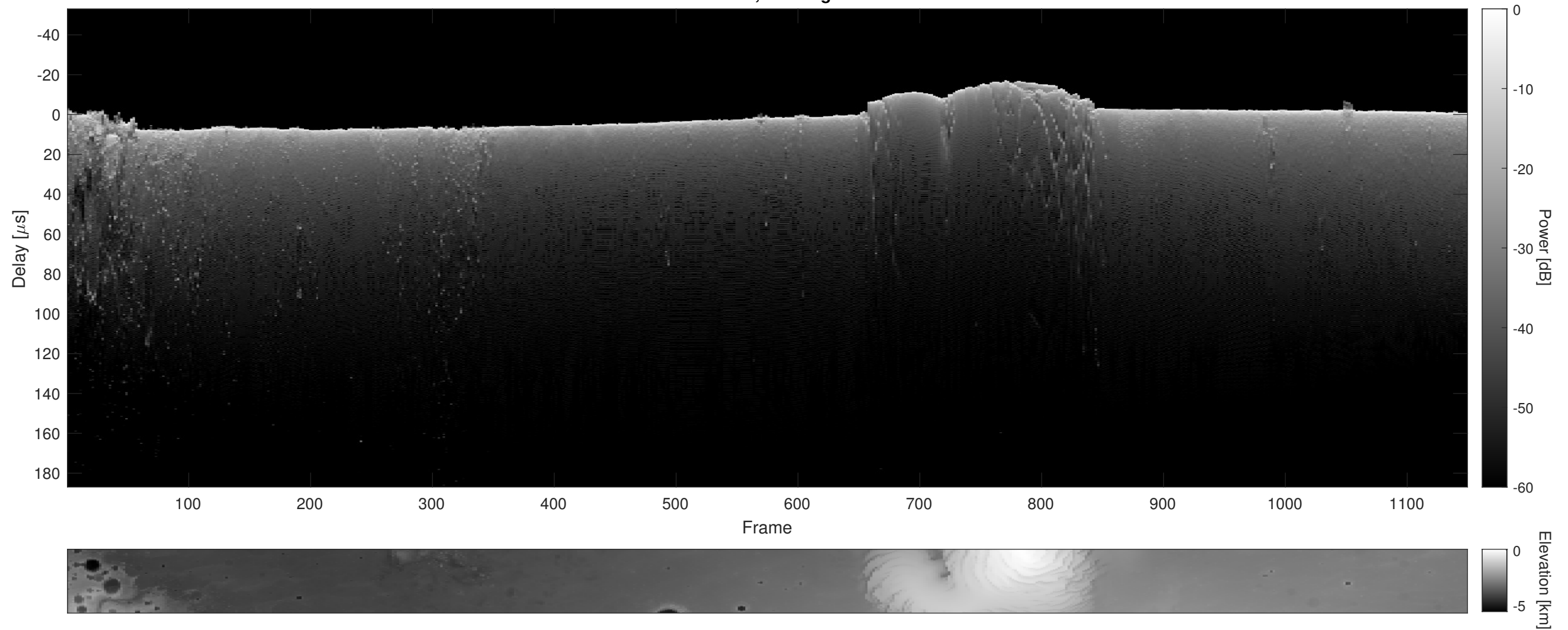
Orbit 9891, Cluttergram
