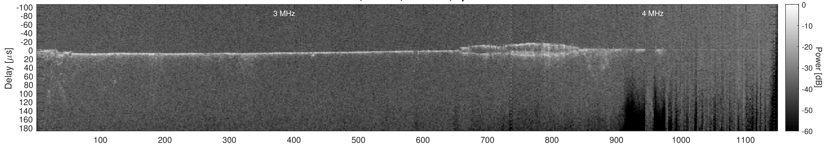
Orbit 9891, Cluttergram
