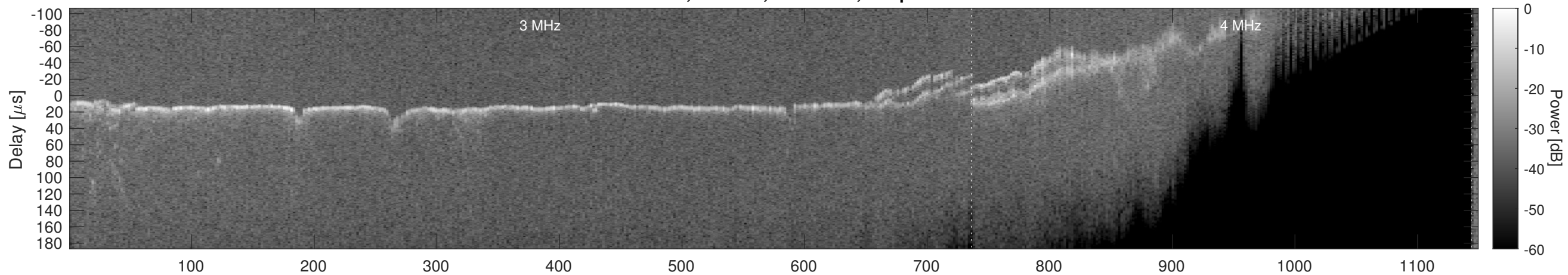
Orbit 9891, Window, Channel 2, Optimized
