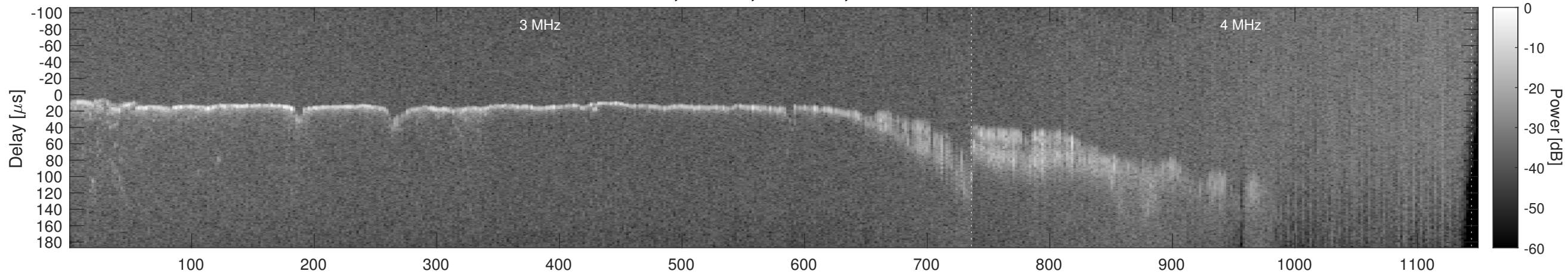
Orbit 9891, Window, Channel 2, Chapman
