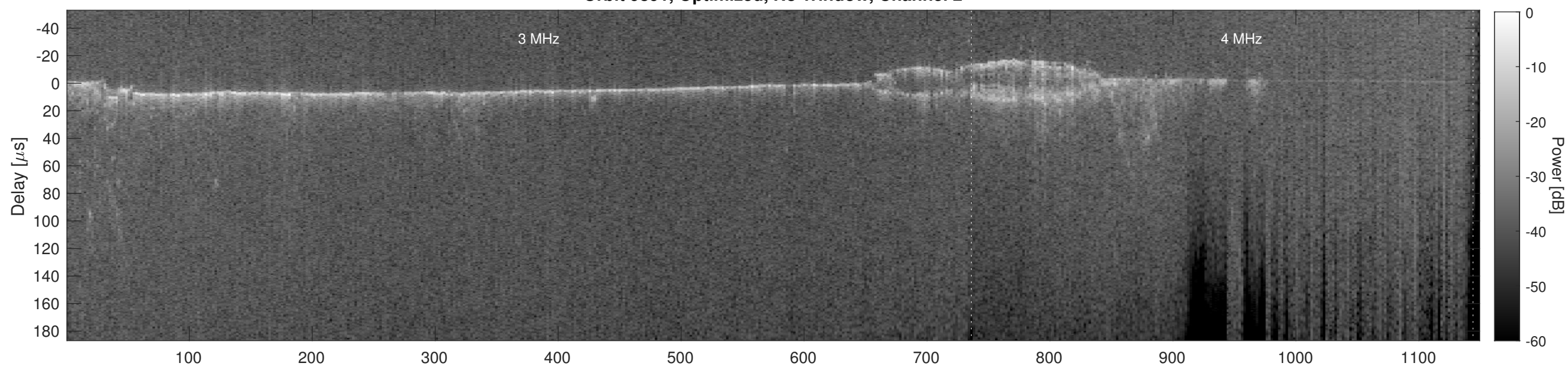
Orbit 9891, Cluttergram
