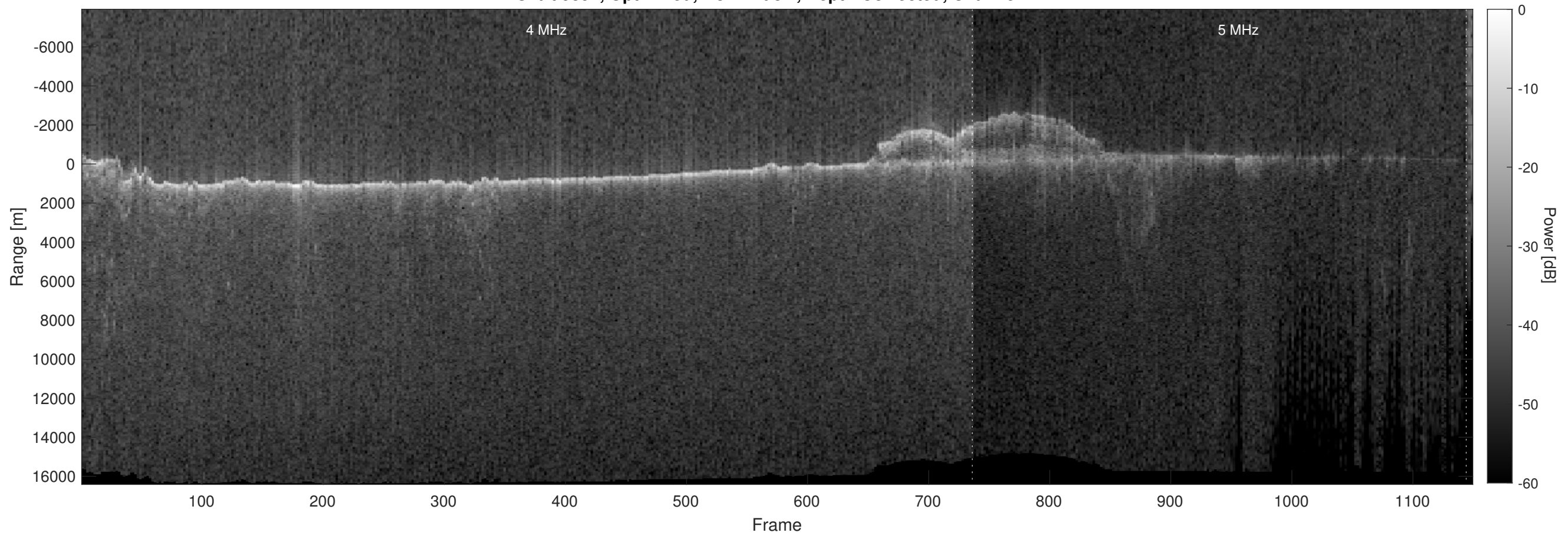
Orbit 9891, Optimized, No Window, Depth-Corrected, Channel 2
