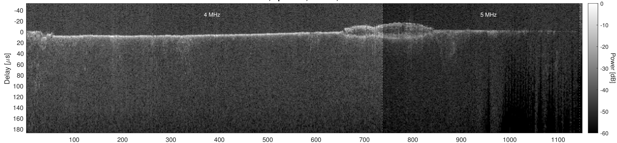
Orbit 9891, Optimized, Window, Channel 2
