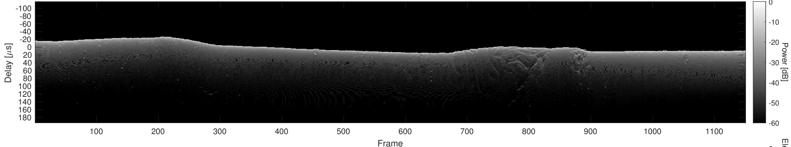
Orbit 9892, Cluttergram
