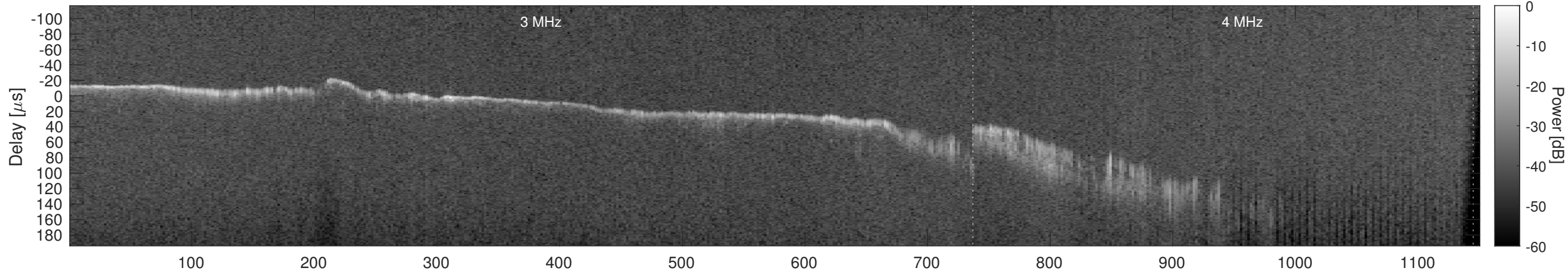
Orbit 9892, Window, Channel 2, Chapman
