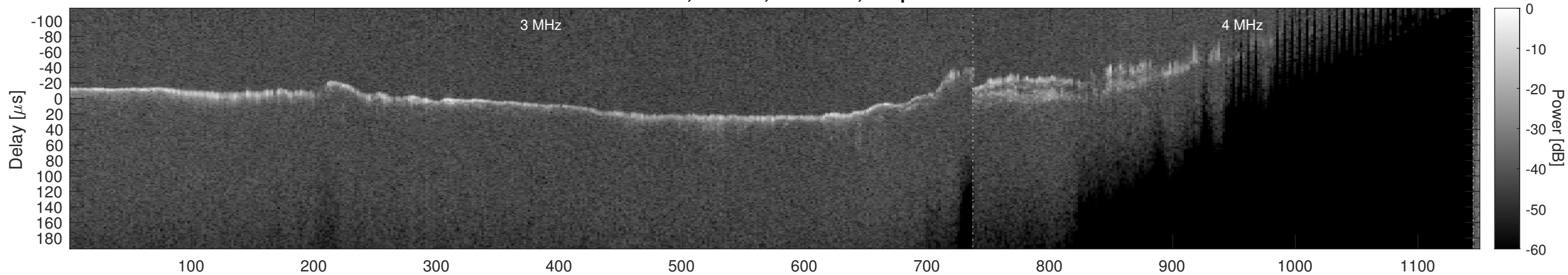
Orbit 9892, Window, Channel 2, Optimized
