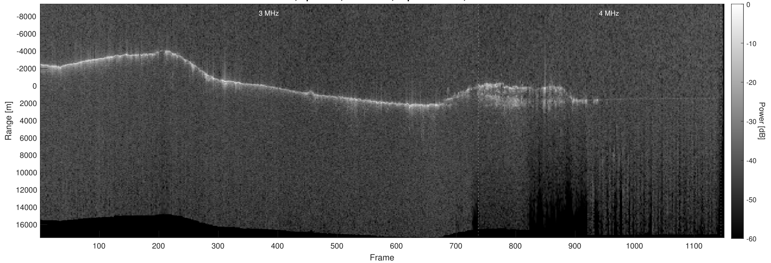
Orbit 9892, Optimized, No Window, Depth-Corrected, Channel 2
