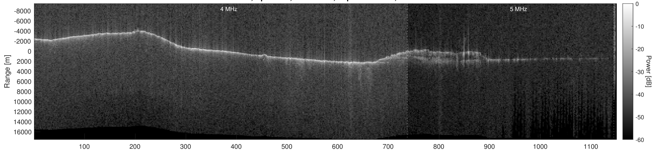
Orbit 9892, Optimized, No Window, Depth-Corrected, Channel 2
