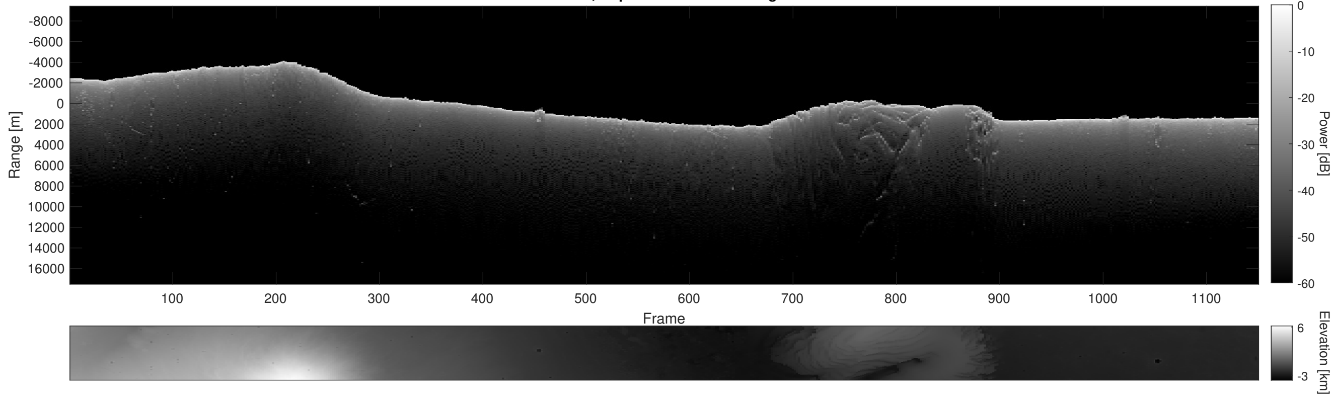
Orbit 9892, Depth-Corrected Cluttergram
