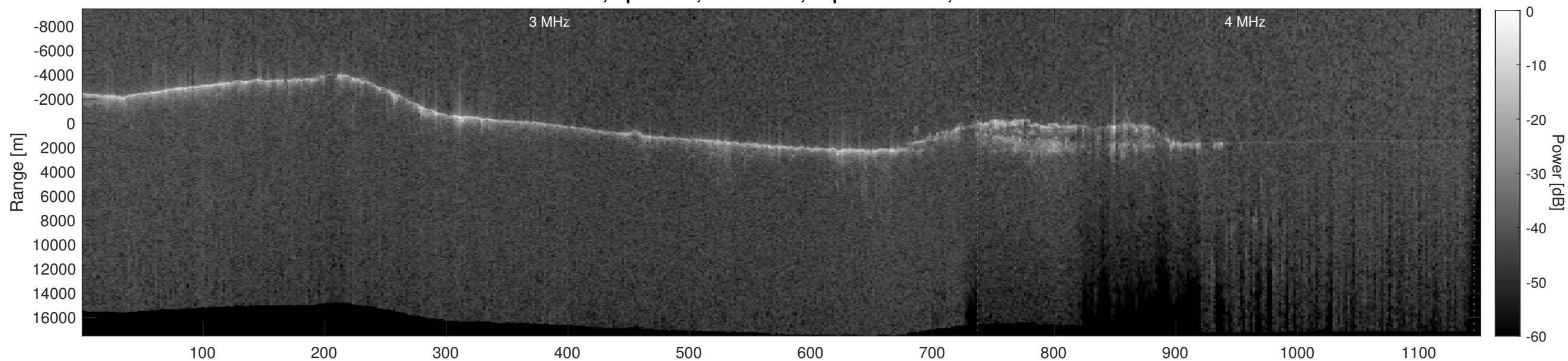
Orbit 9892, Depth-Corrected Cluttergram
