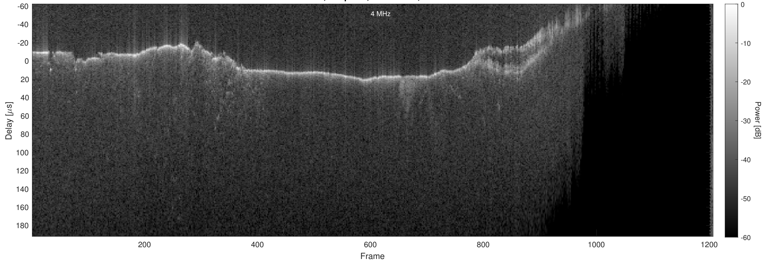
Orbit 9895, Chapman, No Window, Channel 2
