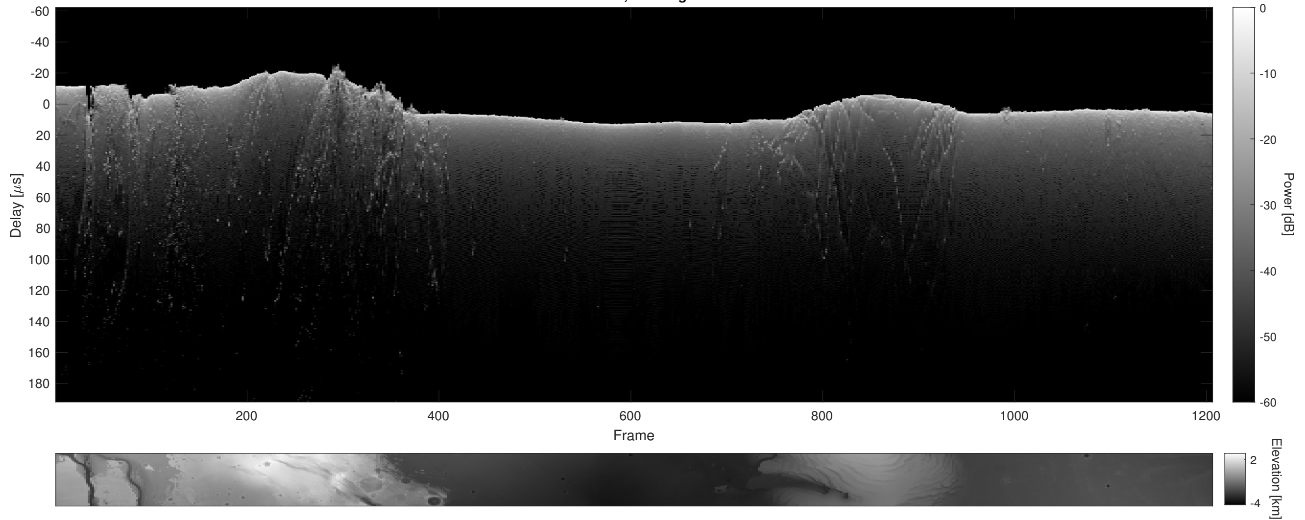
Orbit 9895, Cluttergram
