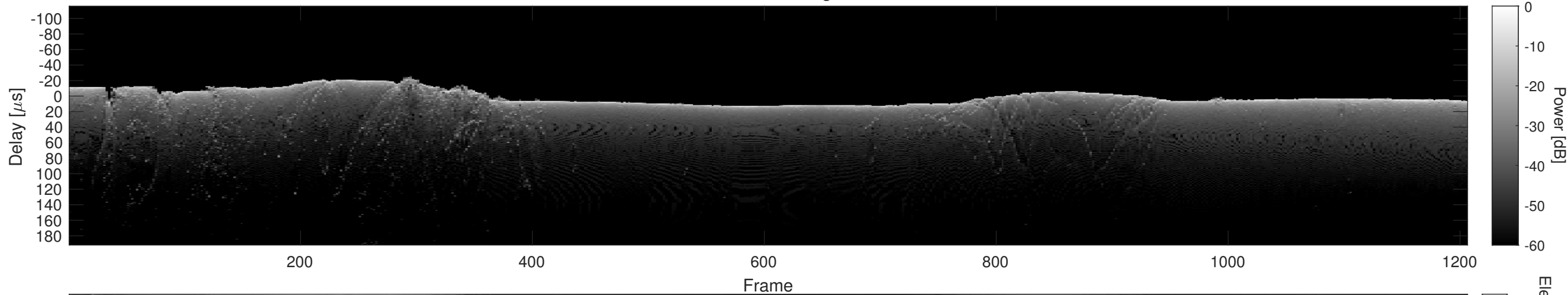
Orbit 9895, Cluttergram
