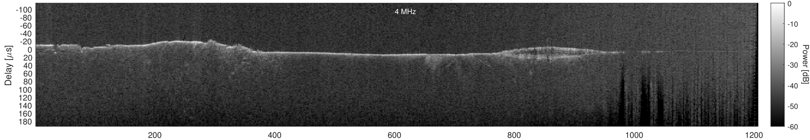
Orbit 9895, Cluttergram
