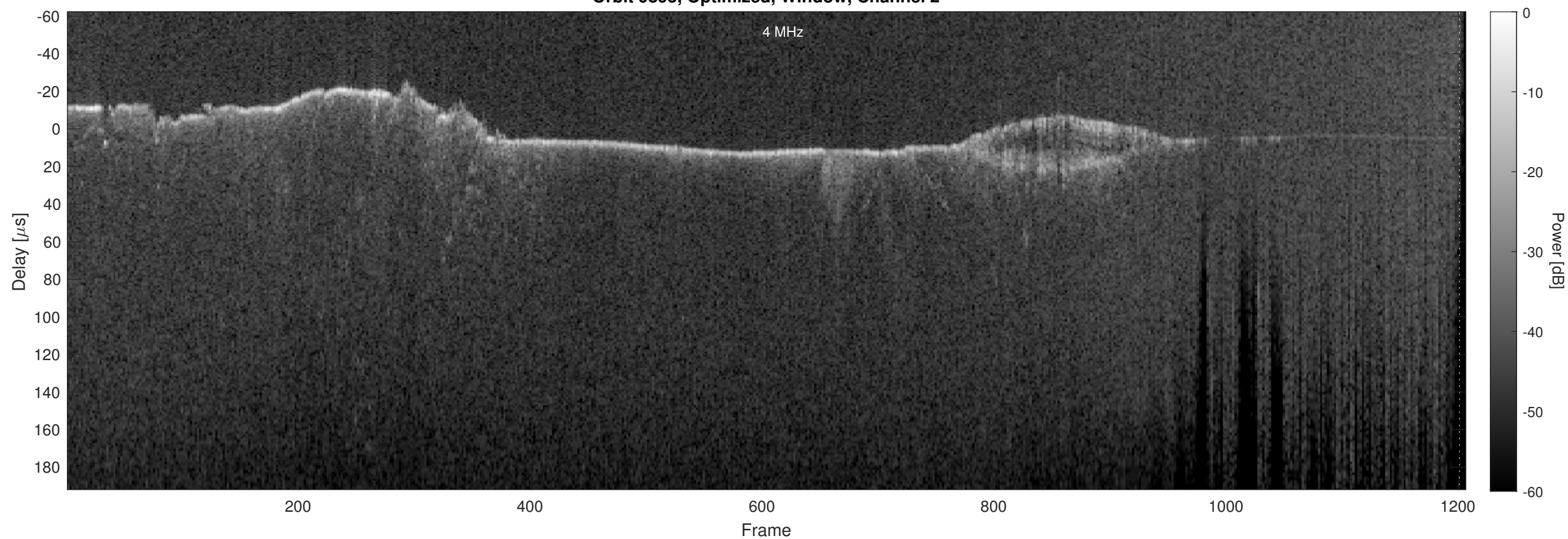
Orbit 9895, Optimized, Window, Channel 2
