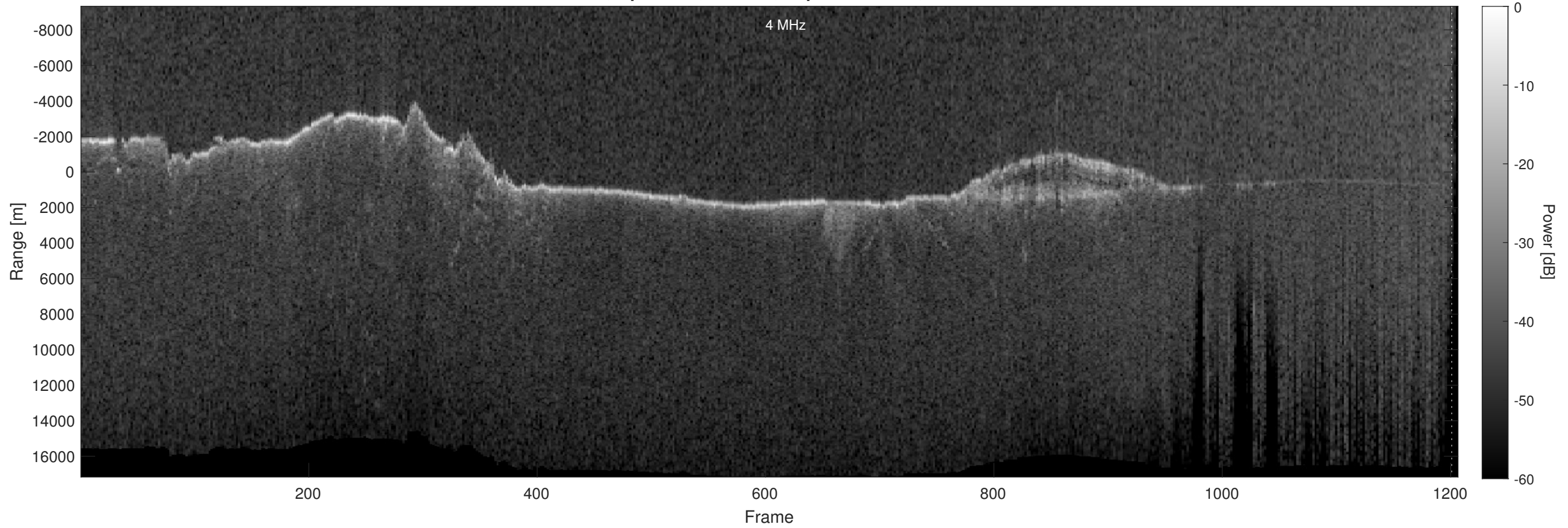
Orbit 9895, Optimized, Window, Depth-Corrected, Channel 2
