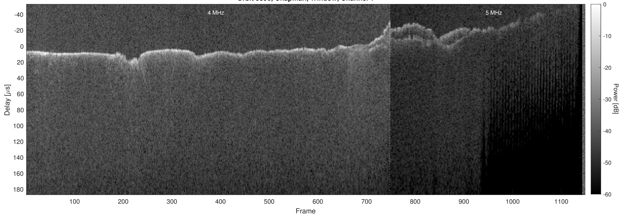
Orbit 9896, Chapman, Window, Channel 2
