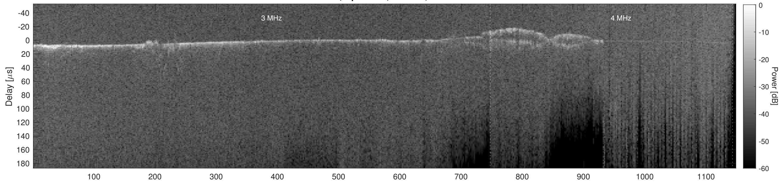
Orbit 9896, Cluttergram
