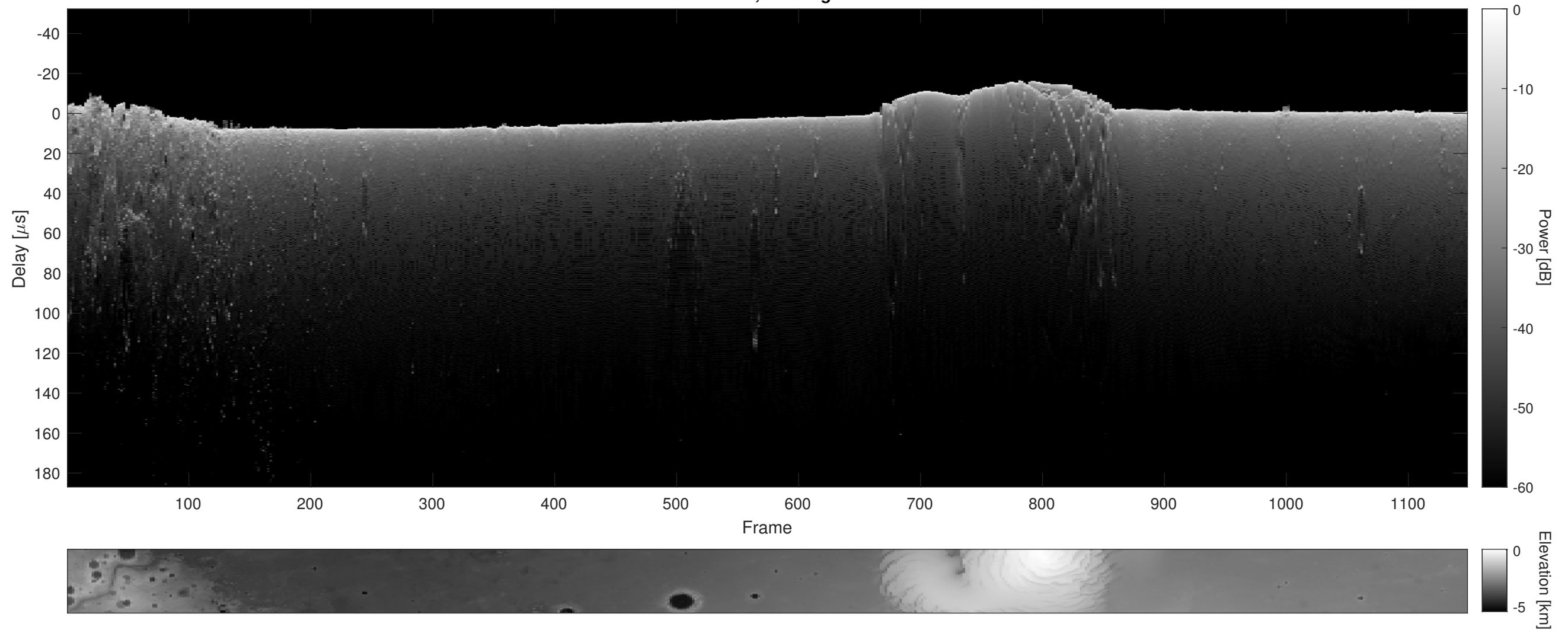
Orbit 9898, Cluttergram
