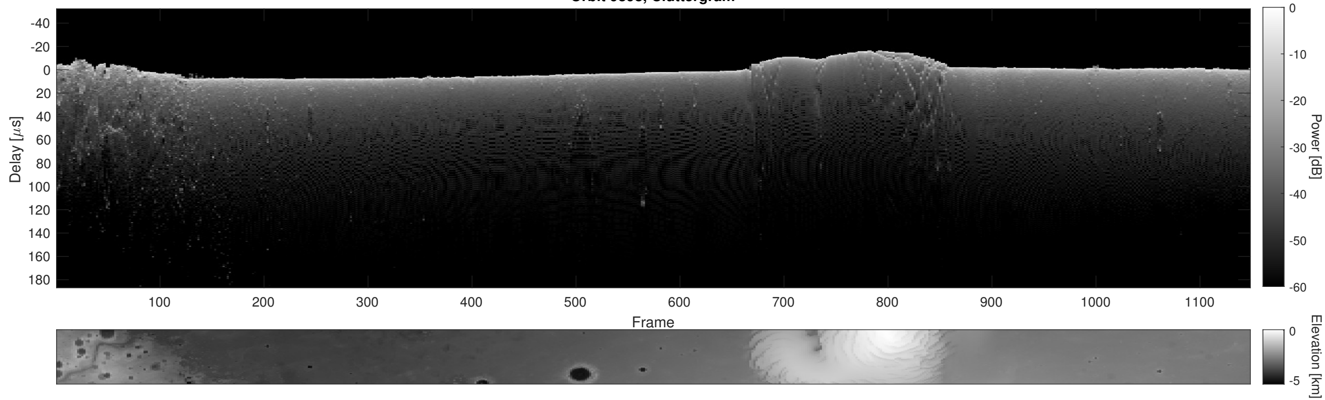
Orbit 9898, Cluttergram
