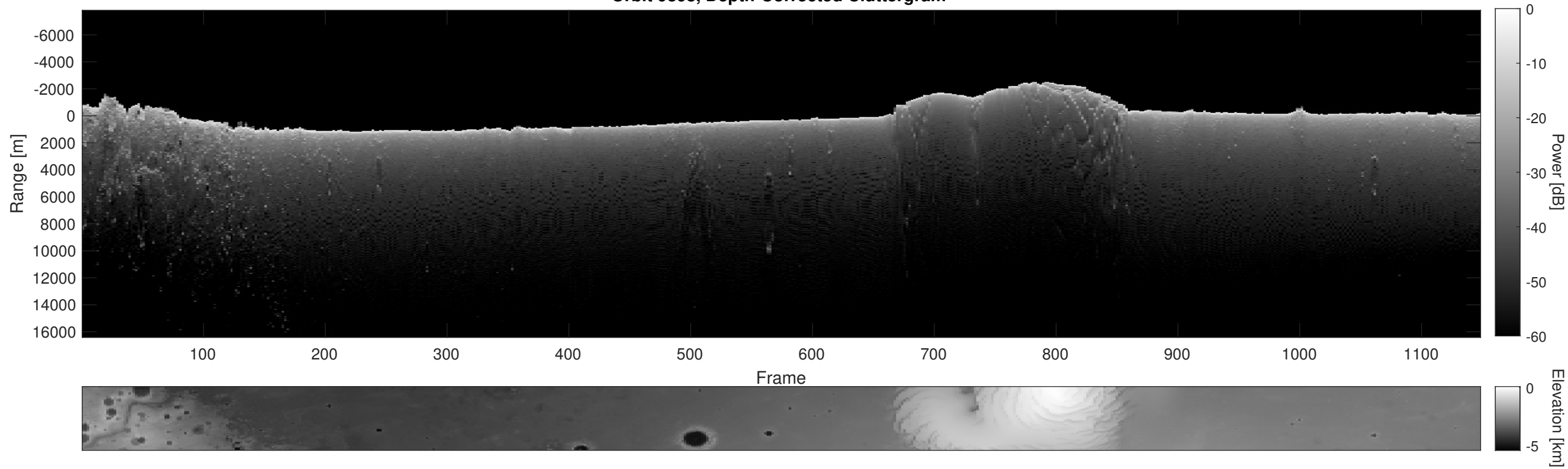
Orbit 9898, Depth-Corrected Cluttergram
