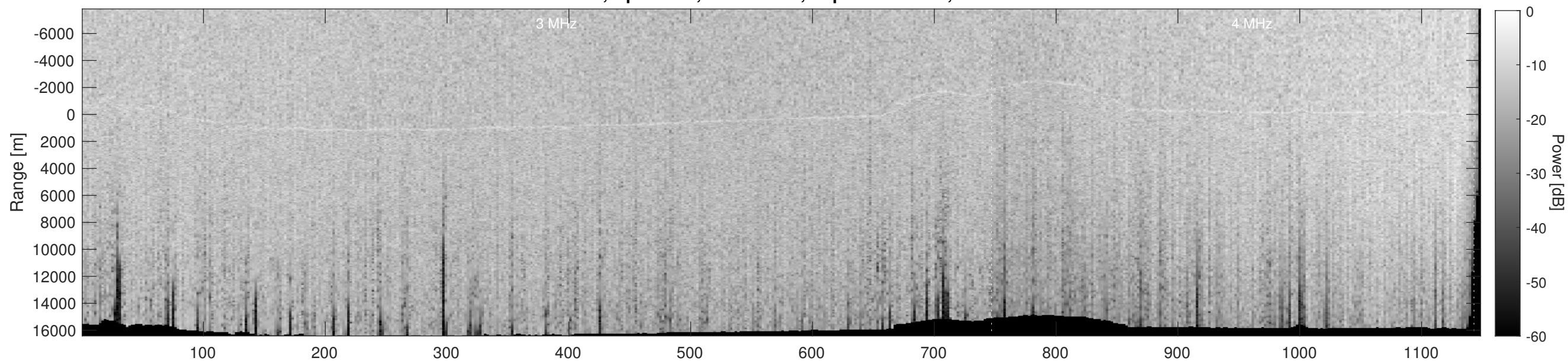
Orbit 9898, Depth-Corrected Cluttergram
