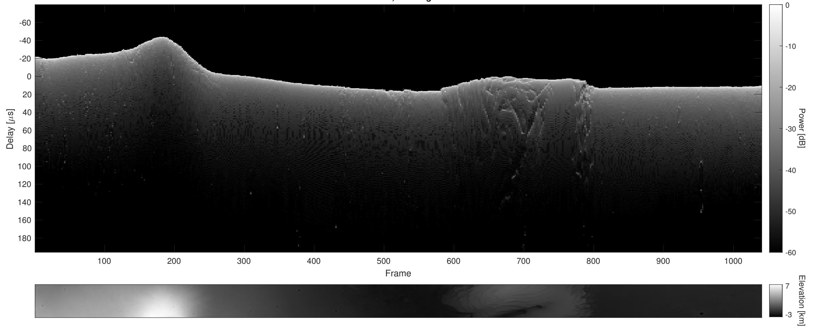
Orbit 9899, Cluttergram
