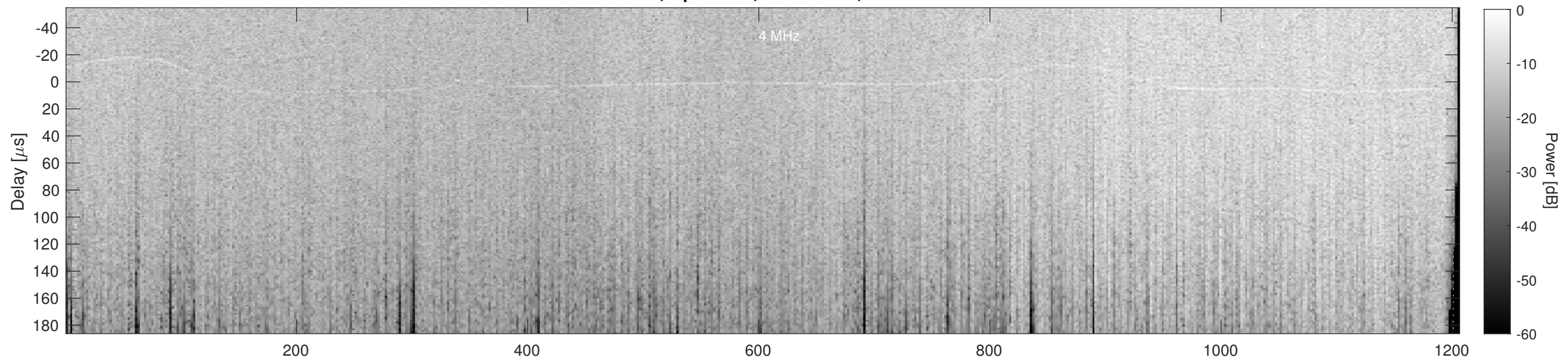
Orbit 9900, Cluttergram
