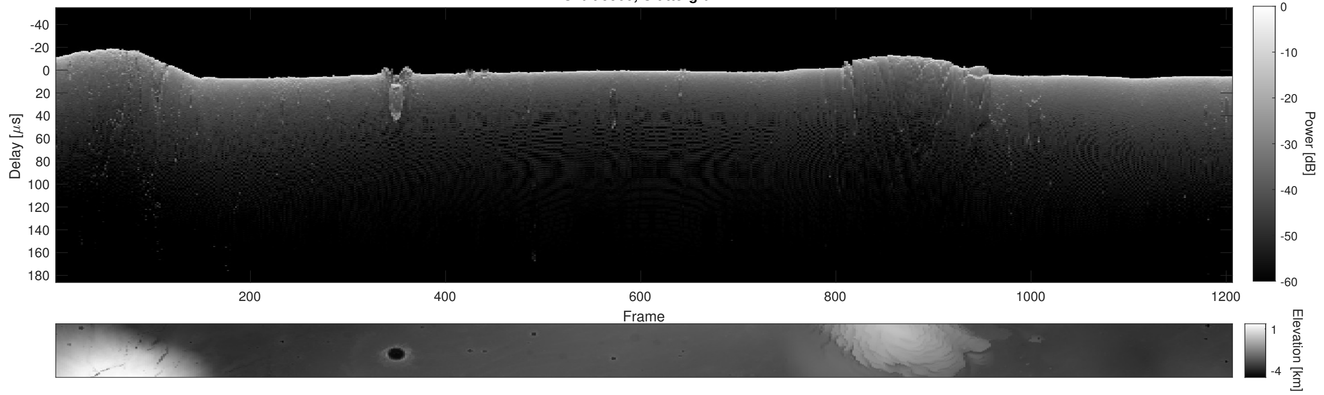
Orbit 9900, Cluttergram
