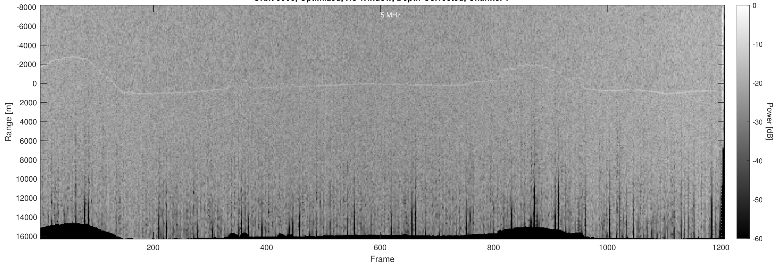
Orbit 9900, Optimized, No Window, Depth-Corrected, Channel 2
