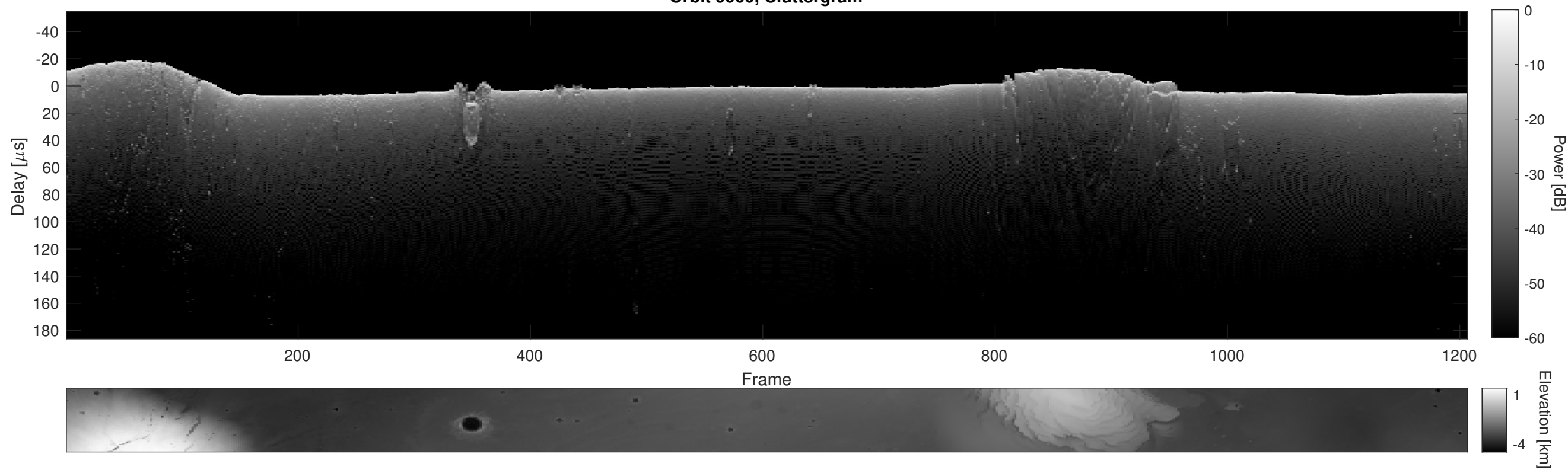
Orbit 9900, Cluttergram
