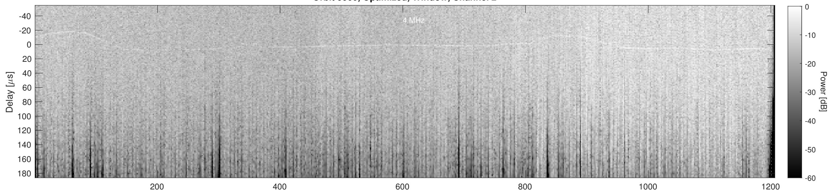
Orbit 9900, Cluttergram
