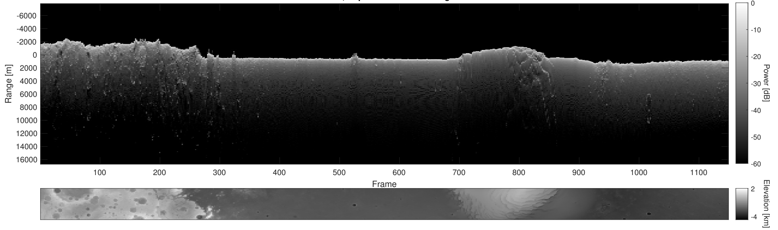
Orbit 9901, Depth-Corrected Cluttergram
