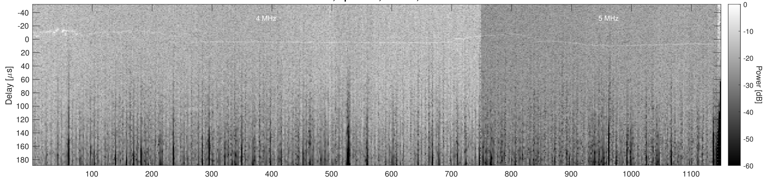
Orbit 9901, Optimized, Window, Channel 2
